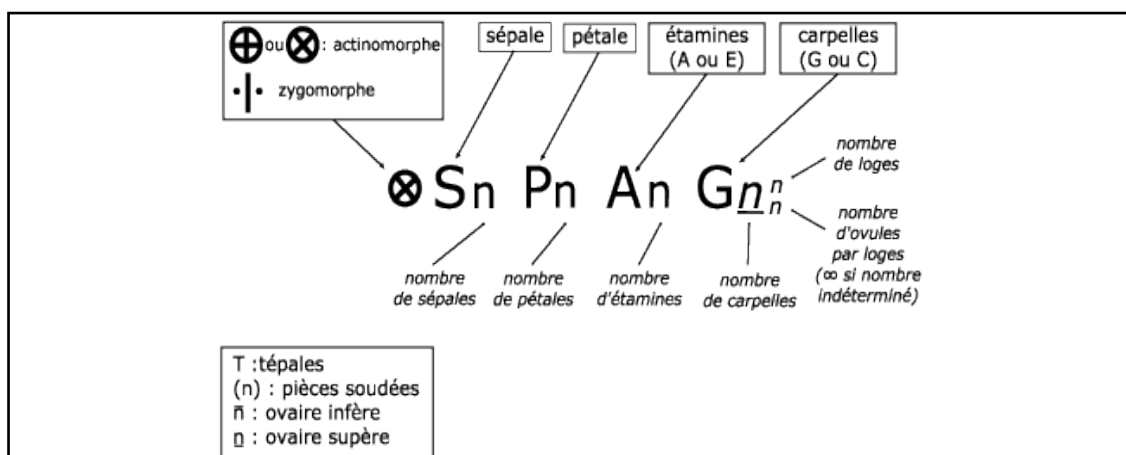
Figure 11: Formule florale
