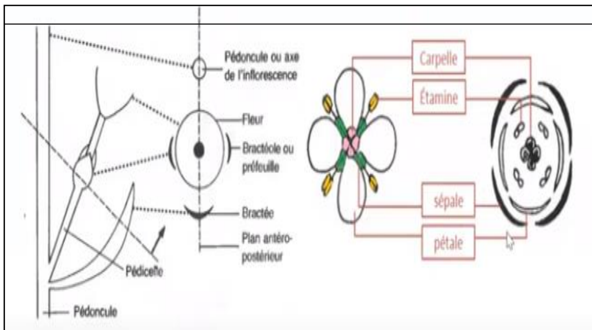
Figure 13 : Diagramme floral
